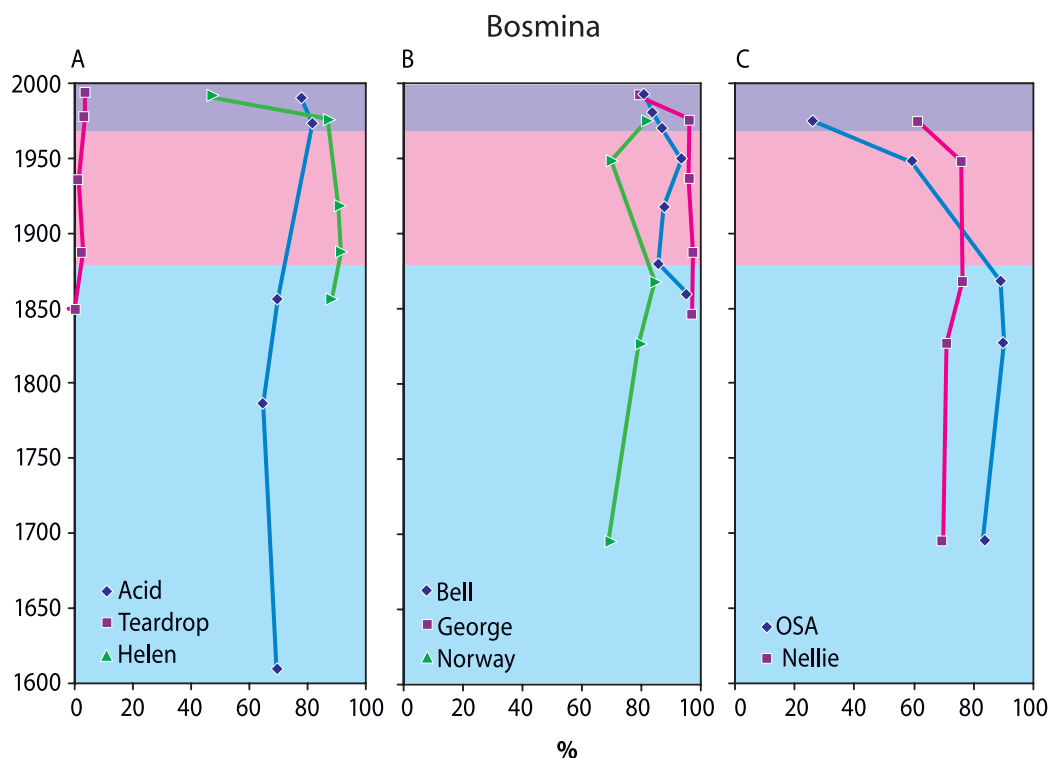
Figure 11. Relative abundance (% of all Cladocera remains) of Bosmina spp. in sediment cores from 8 Killarney lakes. Depth-time profile for the sediment cores were estimated as described in the main text. The main three periods with regard to acidification are indicated with different colours; light blue: pre-acidification period, pink: acidification period, blue: period with chemical recovery. A: Lakes which have never been severely acidified, B: Lakes which have been acidified but have shown a clear chemical recovery, C: Lakes which have been severely acidified and only show a slow chemical recovery.
