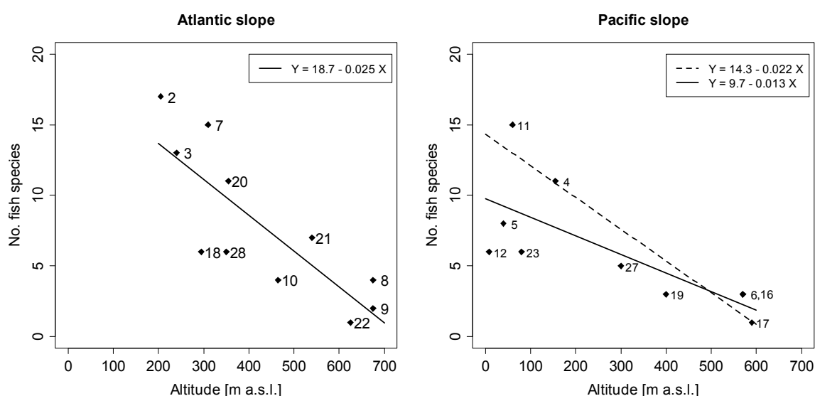
Figure 3 Recorded number of fish species versus altitude in ACG rivers draining to the Atlantic (left) and to the Pacific (right). Numbers on data points refer to locality number in Table 1 and Figure 1. For localities on the Atlantic slope, we have R^2 = 0.67 . For the Pacific slope, the dotted regression line concerns localities with permanent water ( N = 7 ; R^2 = 0.87 ), whereas the bold line represents all localities ( N = 10 ; R^2 = 0.54 ), including the low-lying small watersheds with seasonal water (locs. 5, 12 and 23). All regressions are significant ( p < 0.05 ).
