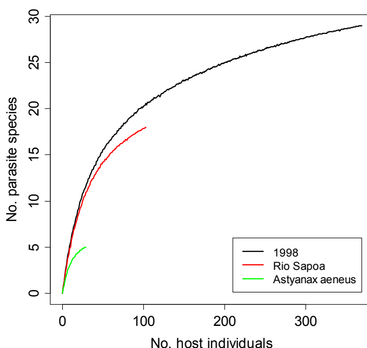
Figure 4 Relation between the number of fish hosts examined and the number of parasite species identified in the samples from 1998. Green curve: all Astyanax aeneus from Rio Sapo (locality 2), red curve: all individuals of all fish species at this locality, and black curve: all fish from all localities surveyed in 1998. The method is described in section 3.4 on p. 12.
